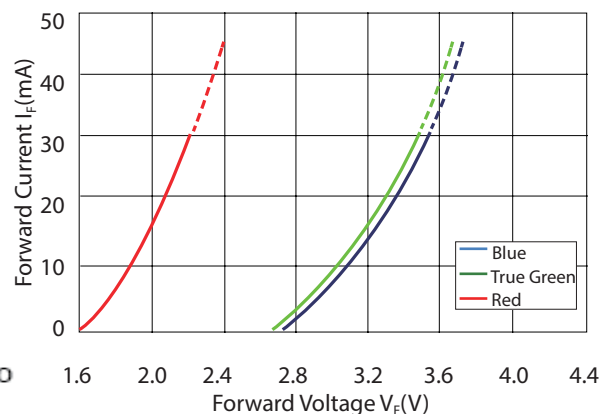
Forward current vs. forward voltage for PLCC 5050 series
