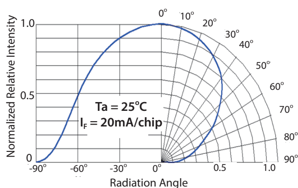
Beam pattern diagram for PLCC 5050 series
