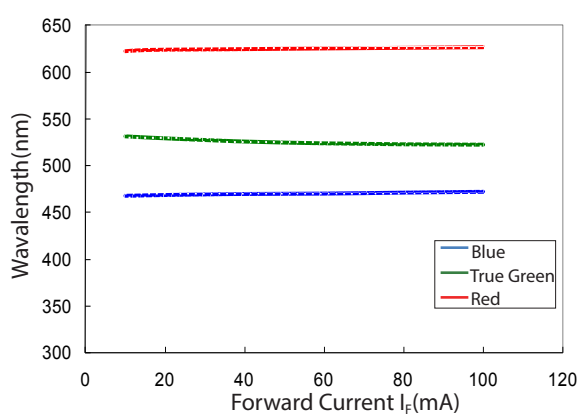
Wavelength vs. Forward Current for PLCC 5050
